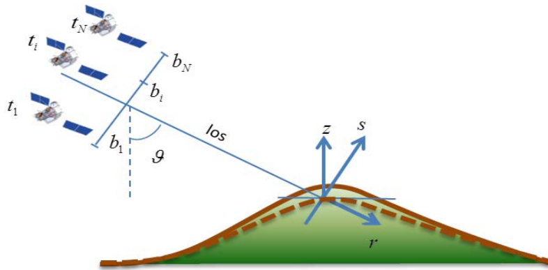
Figure 5: Reference geometry for multipass differential SAR interferometry. Continuous and dashed terrain profiles correspond to the true and available (inaccurate) Digital Elevation Model (DEM).
